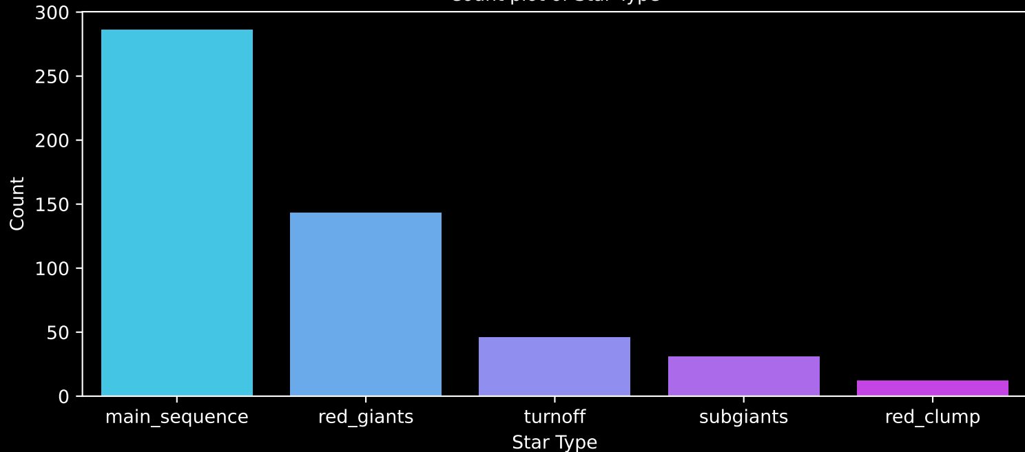
APOGEE DR17 Field: [080+45] Count plot of Star Type
