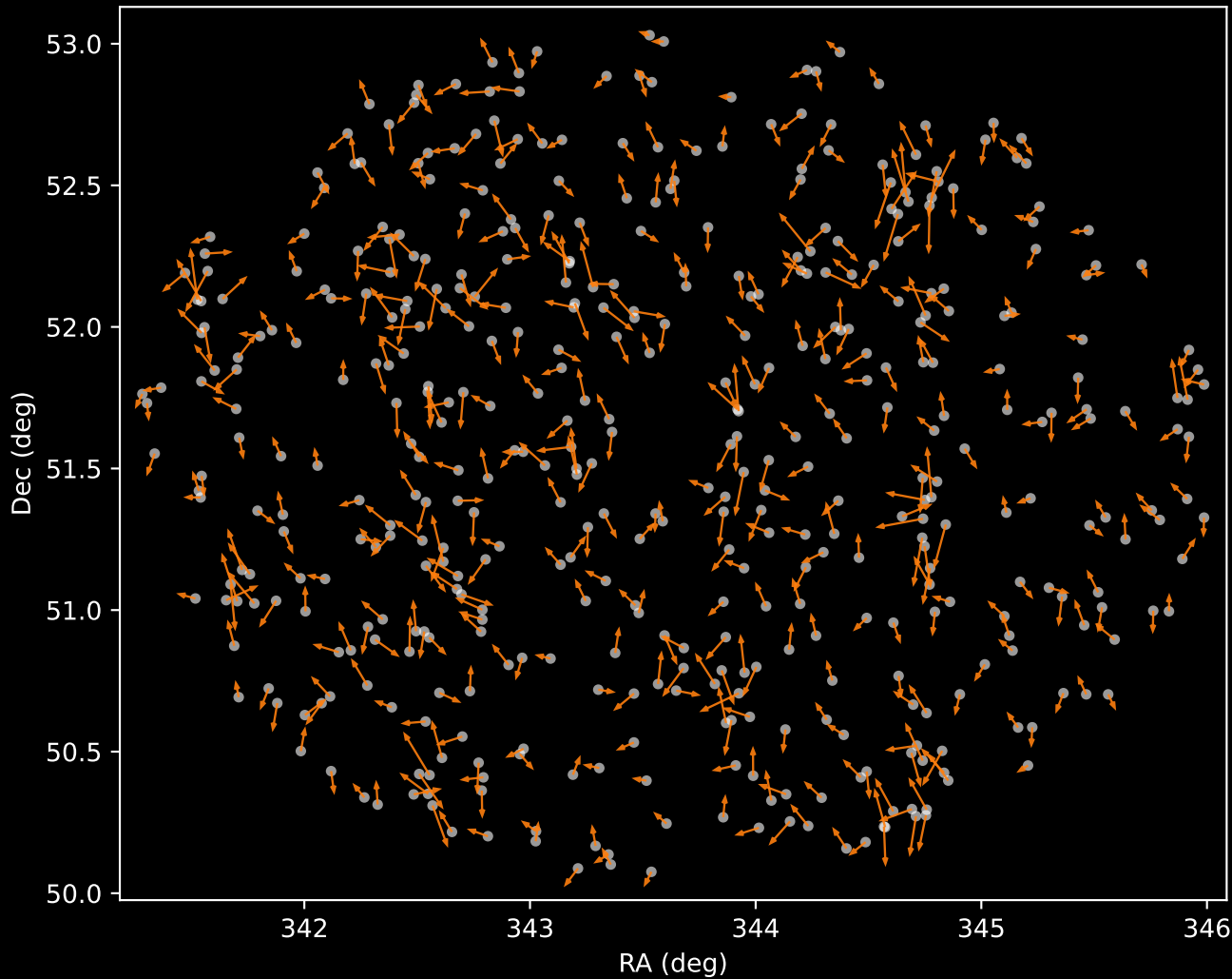
APOGEE DR17 Cluster 2 Proper Motion Vectors (n=463)
