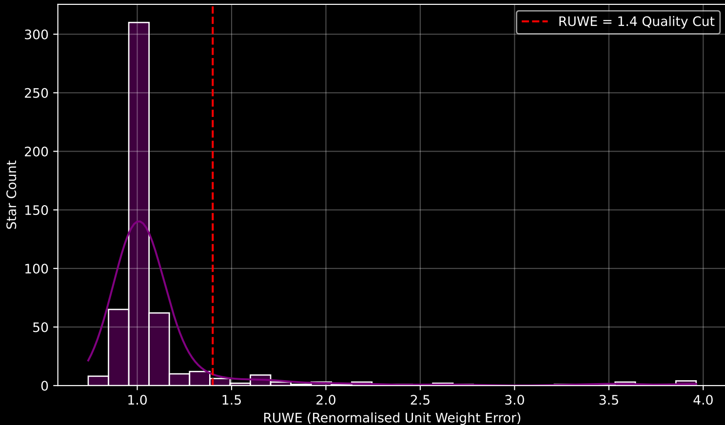
GAPOGEE DR17 Field [080+45] RUWE Distribution (n= 509)
