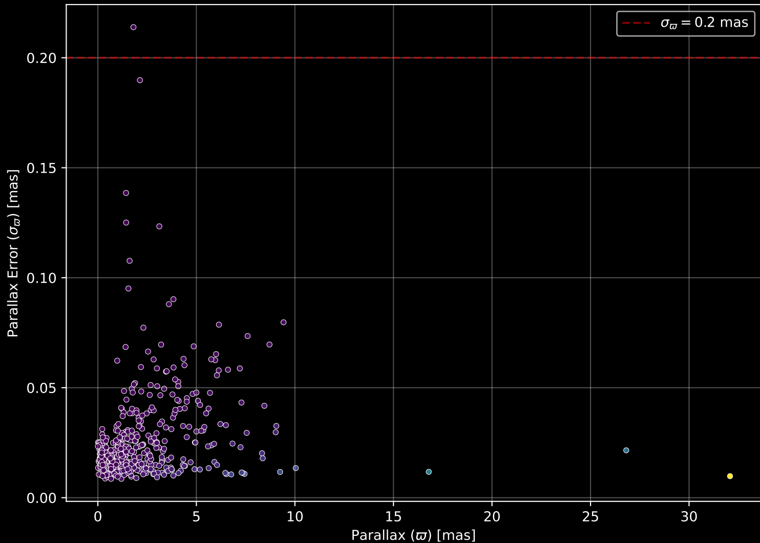
APOGEE DR17 Field: [080+45] Parallax Quality (n= 518)
