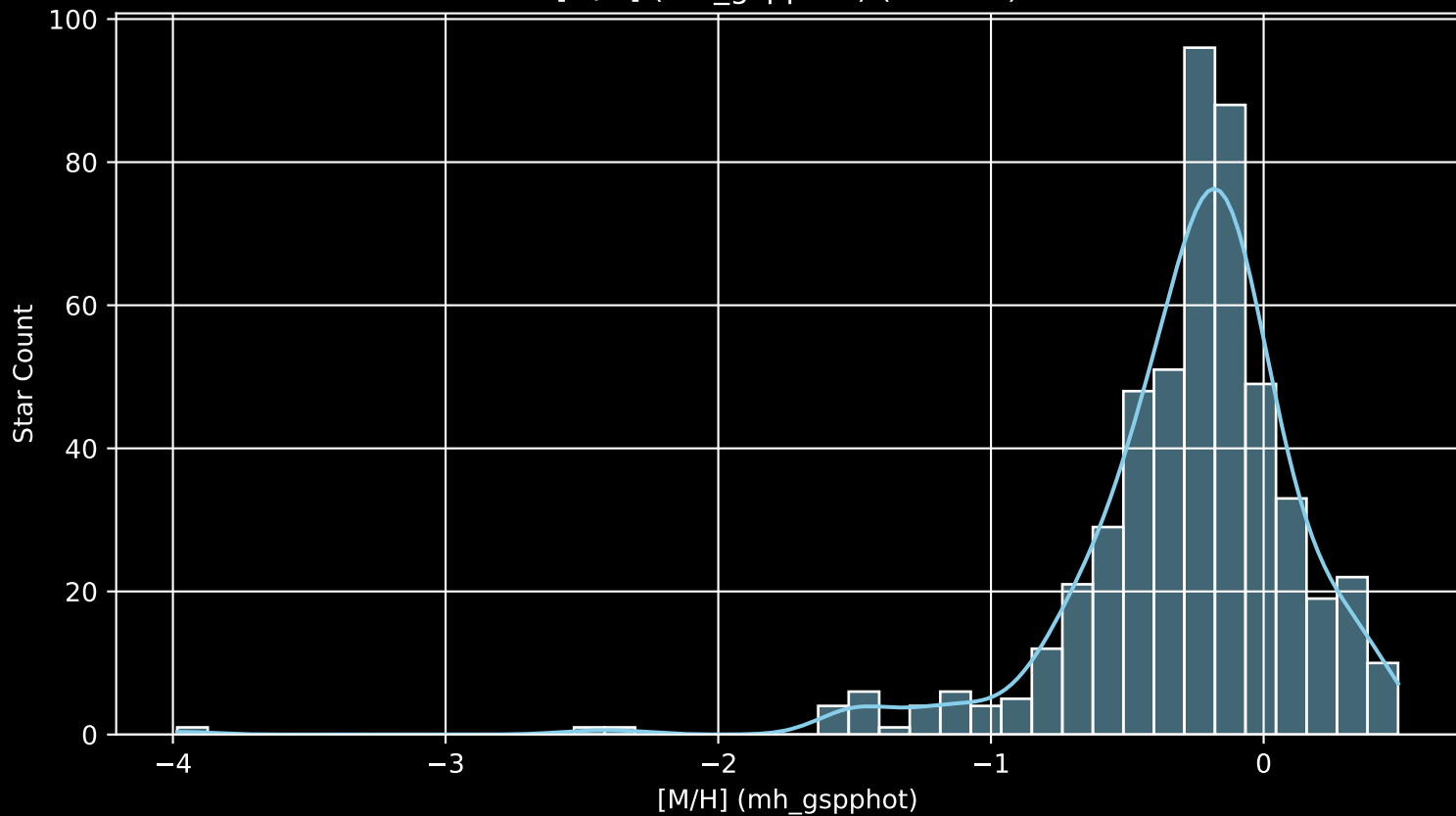
APOGEE DR17 Field: [080+45 [M/H] (mh_gspphot) (n= 511)
