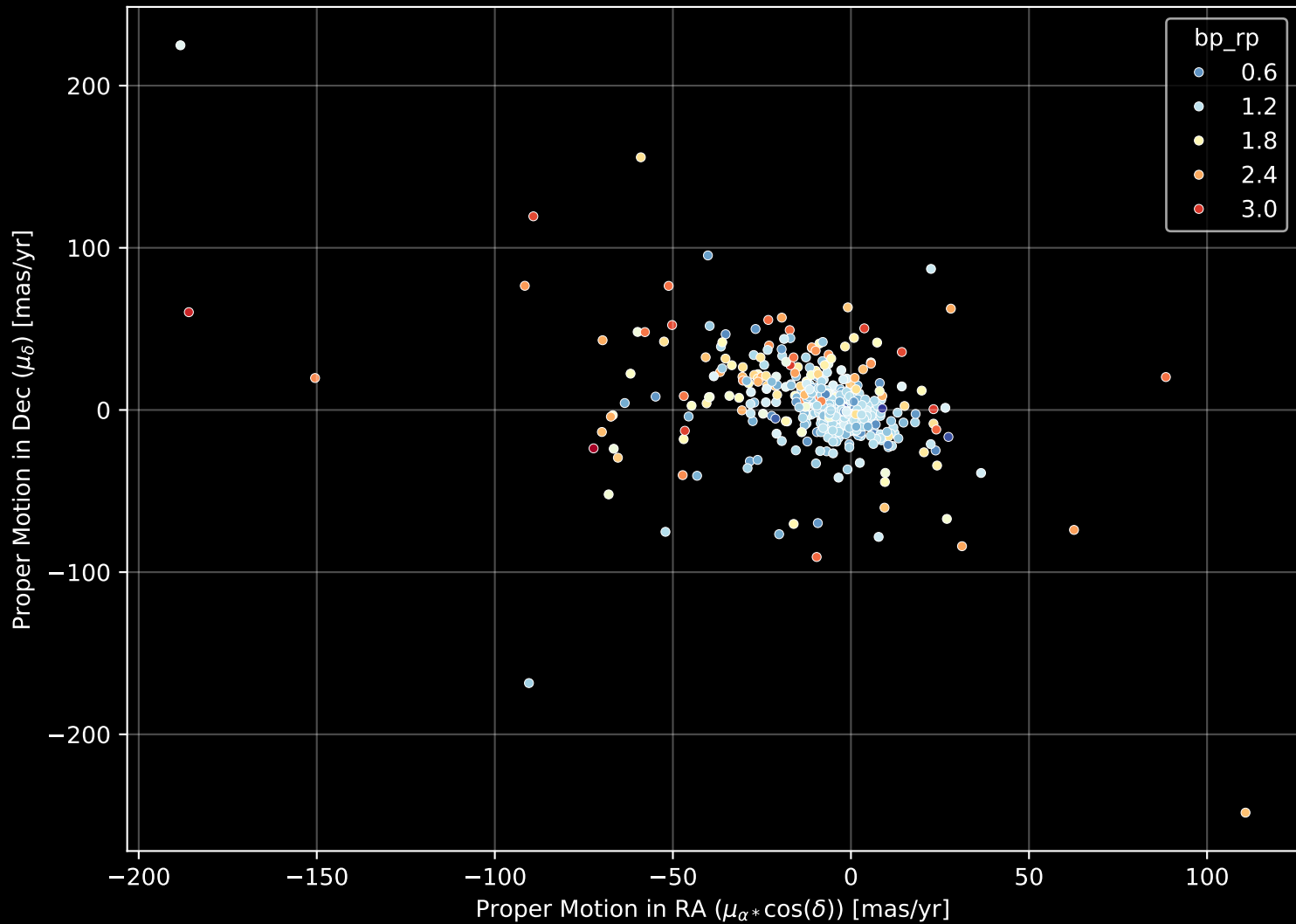
APOGEE DR17 Field: [080+45] Proper Motion Diagram (n= 518)
